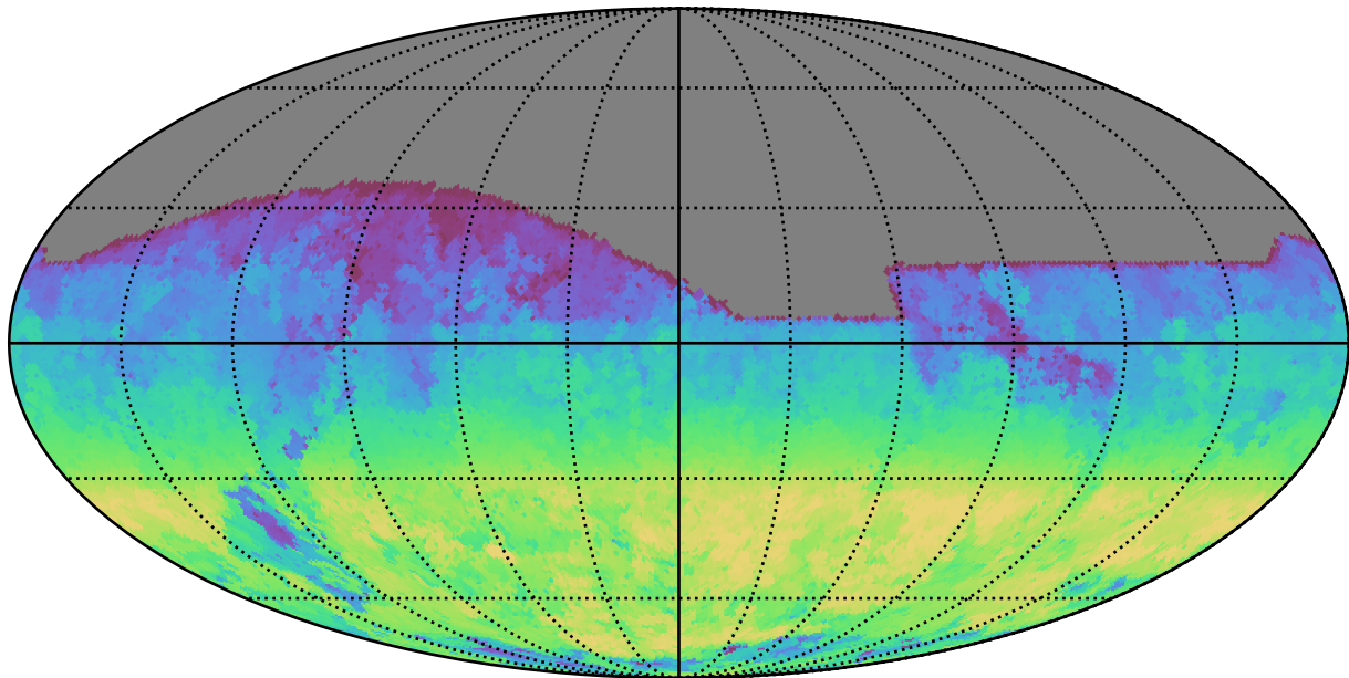
too_5_4v3.4_10yrs All sky z band: AngleRange rotSkyPos
