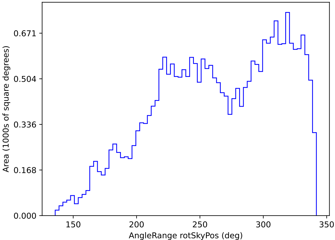
too_5_4v3.4_10yrs All sky z band: AngleRange rotSkyPos
