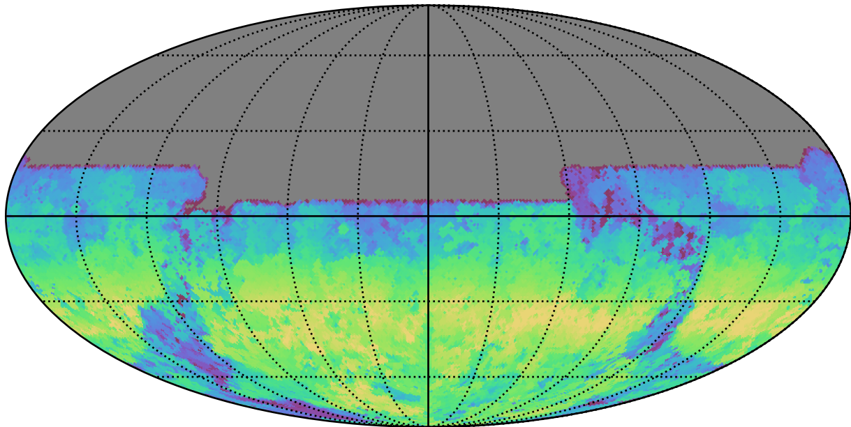
too_5_4v3.4_10yrs All sky u band: AngleRange rotSkyPos
