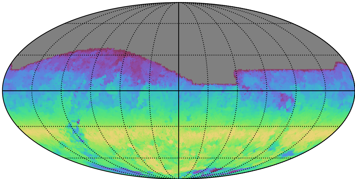
too_5_4v3.4_10yrs All sky r band: AngleRange rotSkyPos
