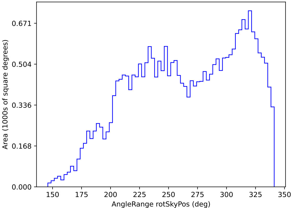
too_5_4v3.4_10yrs All sky i band: AngleRange rotSkyPos
