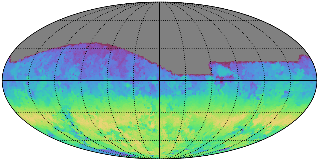
too_5_4v3.4_10yrs All sky g band: AngleRange rotSkyPos
