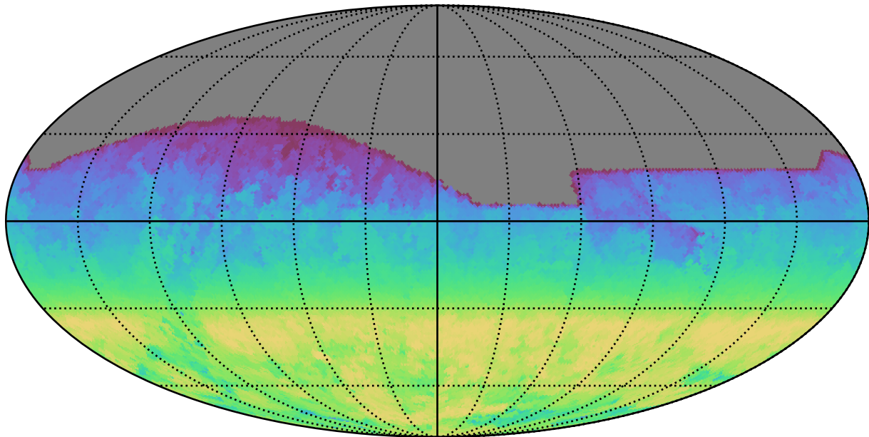
too_5_4v3.4_10yrs All sky all bands: AngleRange rotSkyPos
