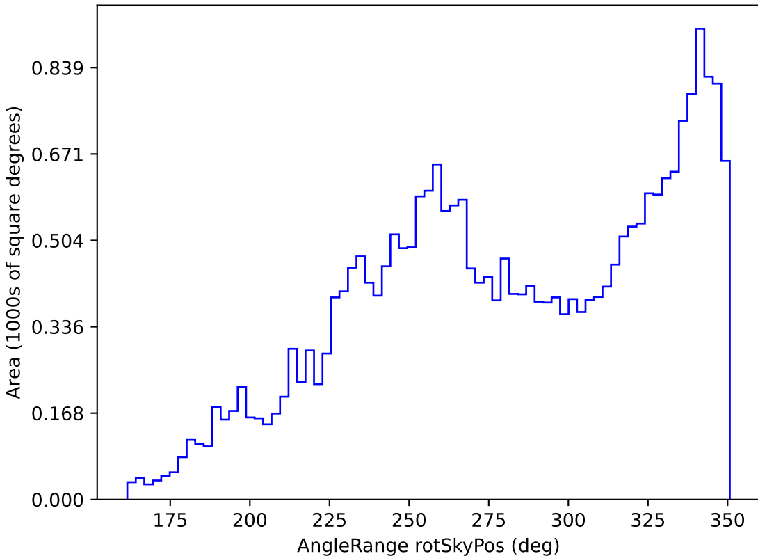
too_5_4v3.4_10yrs All sky all bands: AngleRange rotSkyPos
