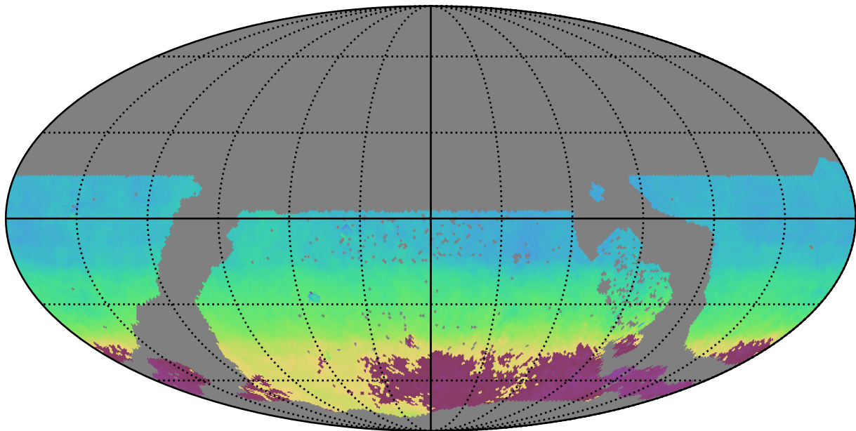
too_5_4v3.4_10yrs WFD z band: AngleMean rotSkyPos
