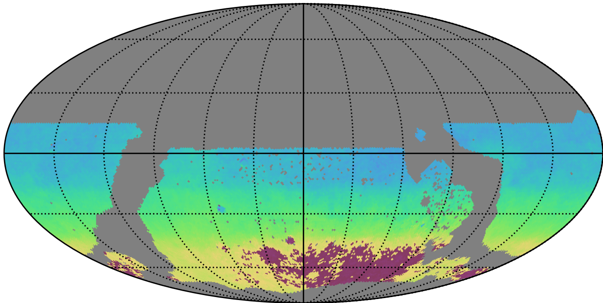
too_5_4v3.4_10yrs WFD y band: AngleMean rotSkyPos
