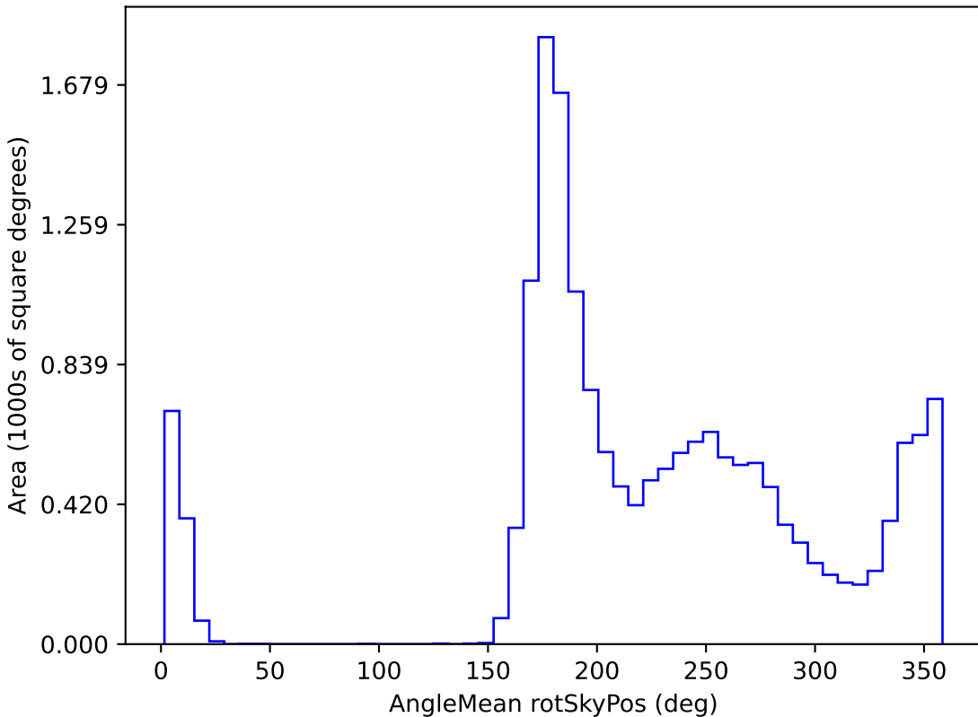
too_5_4v3.4_10yrs WFD y band: AngleMean rotSkyPos
