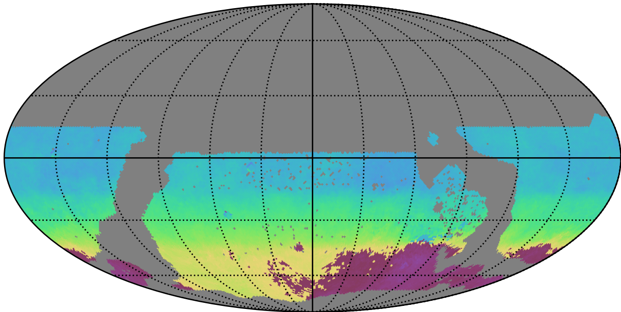
too_5_4v3.4_10yrs WFD r band: AngleMean rotSkyPos
