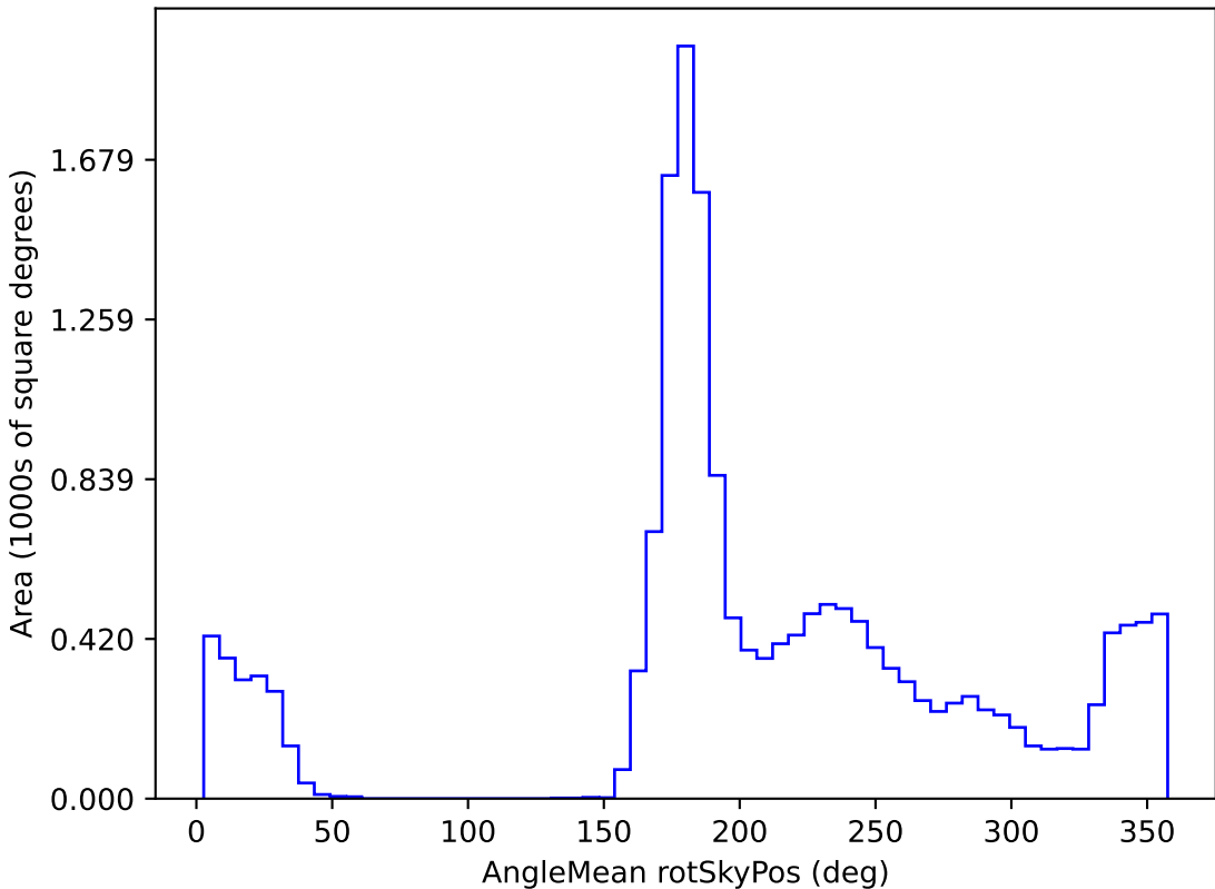
too_5_4v3.4_10yrs WFD r band: AngleMean rotSkyPos
