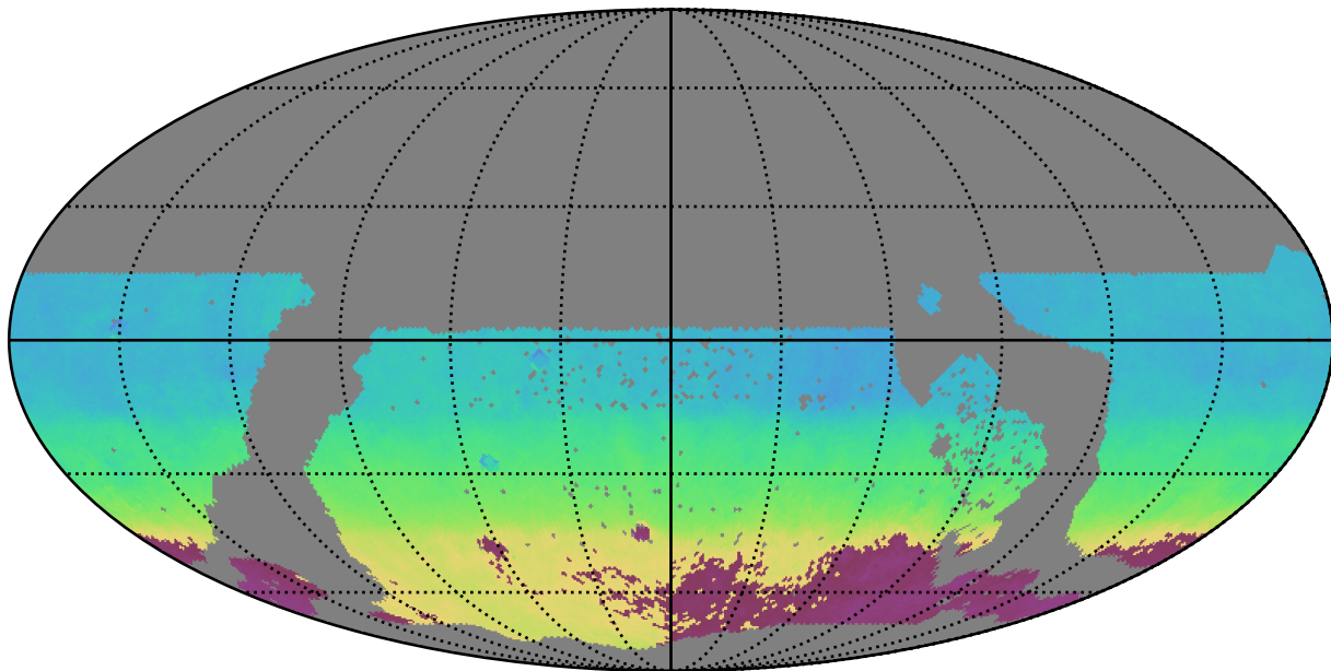
too_5_4v3.4_10yrs WFD i band: AngleMean rotSkyPos
