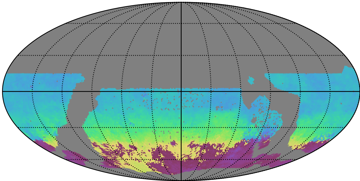
too_5_4v3.4_10yrs WFD g band: AngleMean rotSkyPos
