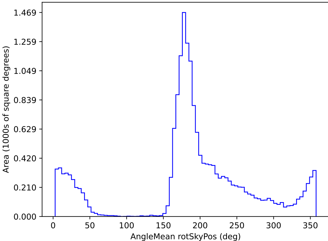
too_5_4v3.4_10yrs WFD g band: AngleMean rotSkyPos
