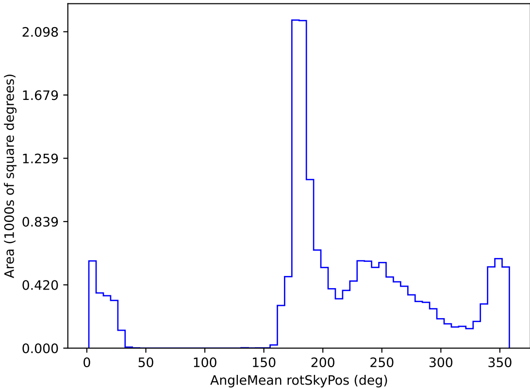
too_5_4v3.4_10yrs WFD all bands: AngleMean rotSkyPos
