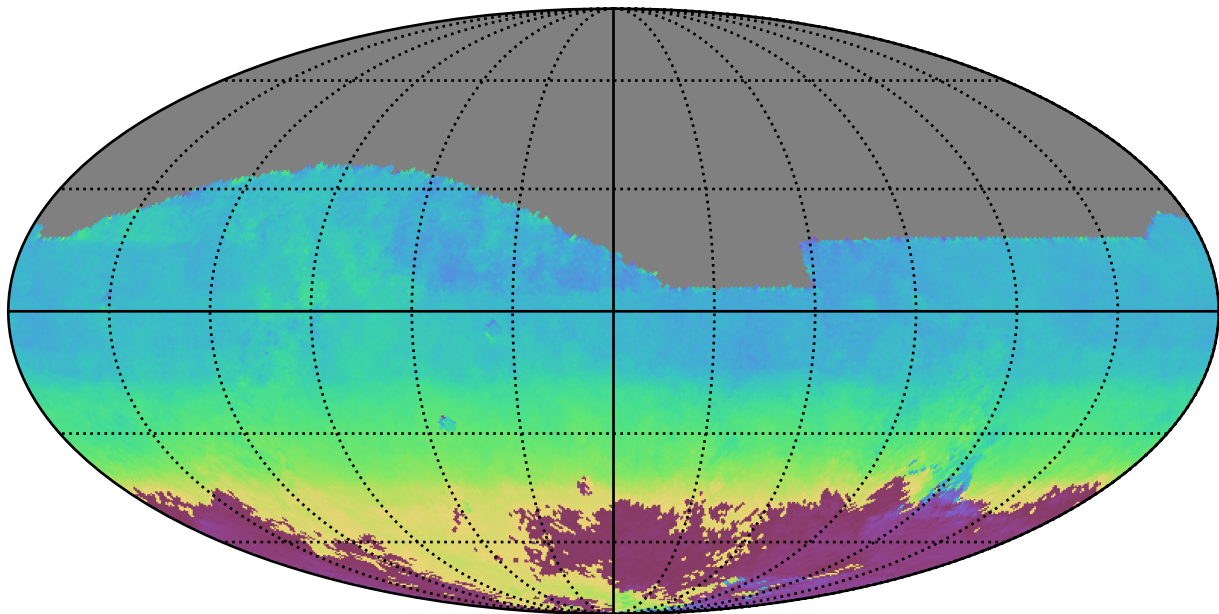
too_5_4v3.4_10yrs All sky z band: AngleMean rotSkyPos
