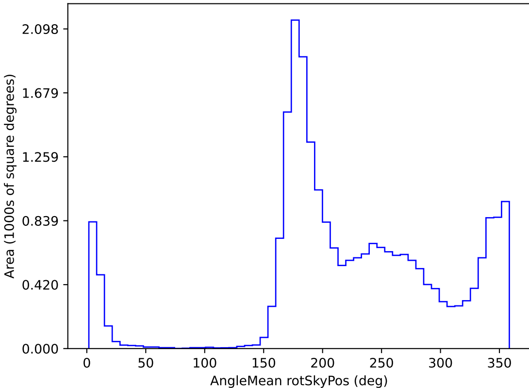
too_5_4v3.4_10yrs All sky y band: AngleMean rotSkyPos
