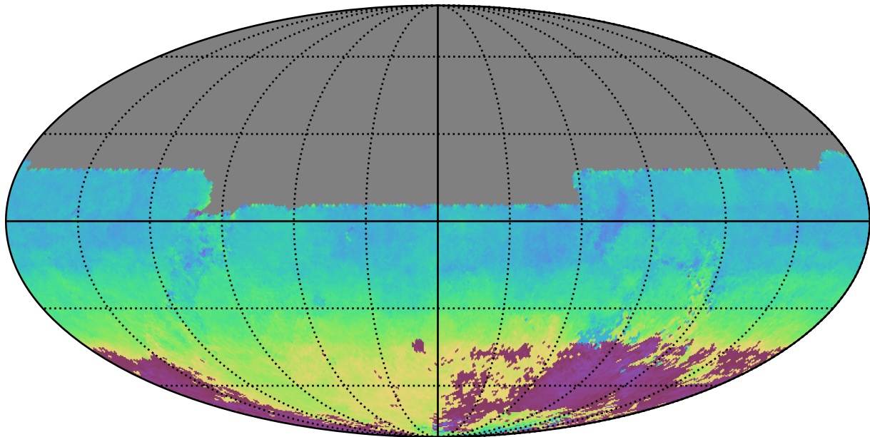
too_5_4v3.4_10yrs All sky u band: AngleMean rotSkyPos
