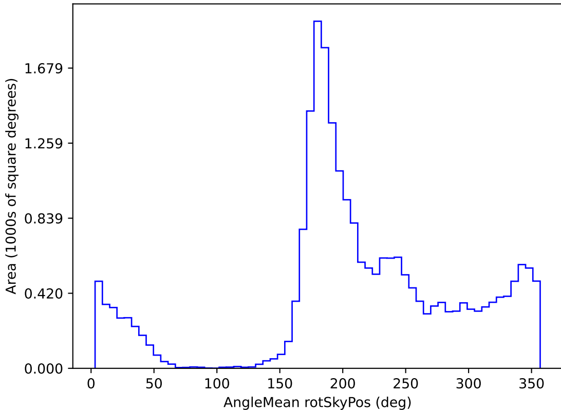
too_5_4v3.4_10yrs All sky u band: AngleMean rotSkyPos
