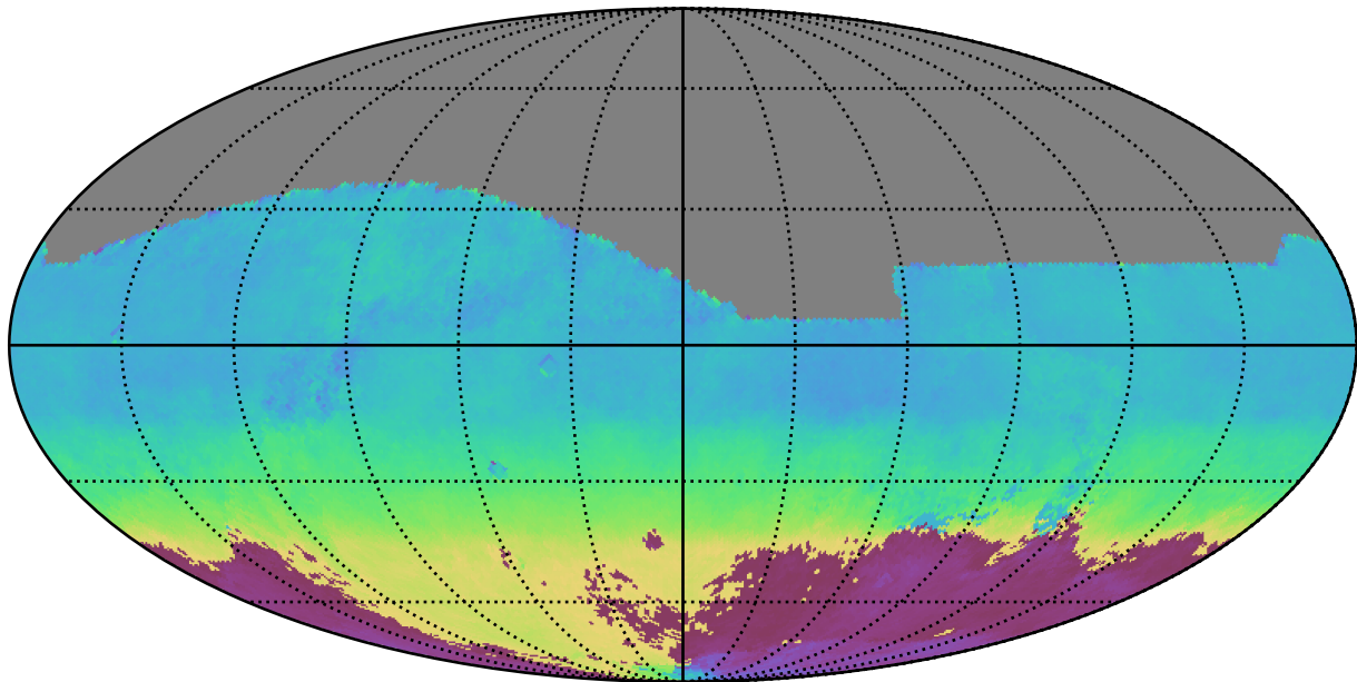
too_5_4v3.4_10yrs All sky r band: AngleMean rotSkyPos
