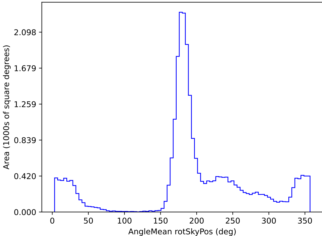
too_5_4v3.4_10yrs All sky r band: AngleMean rotSkyPos
