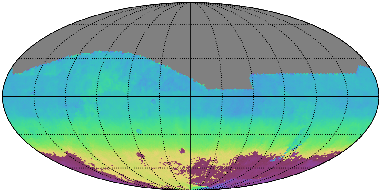
too_5_4v3.4_10yrs All sky i band: AngleMean rotSkyPos
