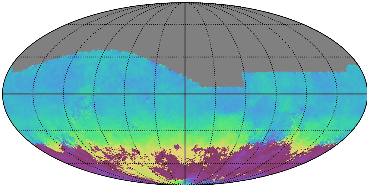
too_5_4v3.4_10yrs All sky g band: AngleMean rotSkyPos
