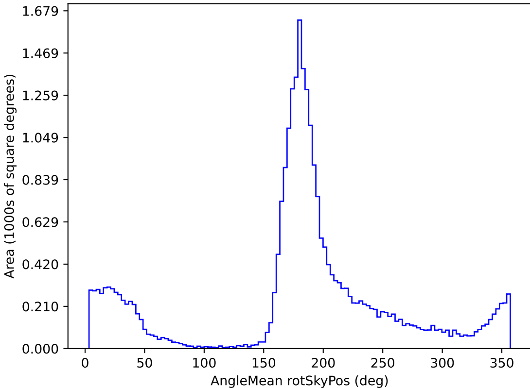
too_5_4v3.4_10yrs All sky g band: AngleMean rotSkyPos
