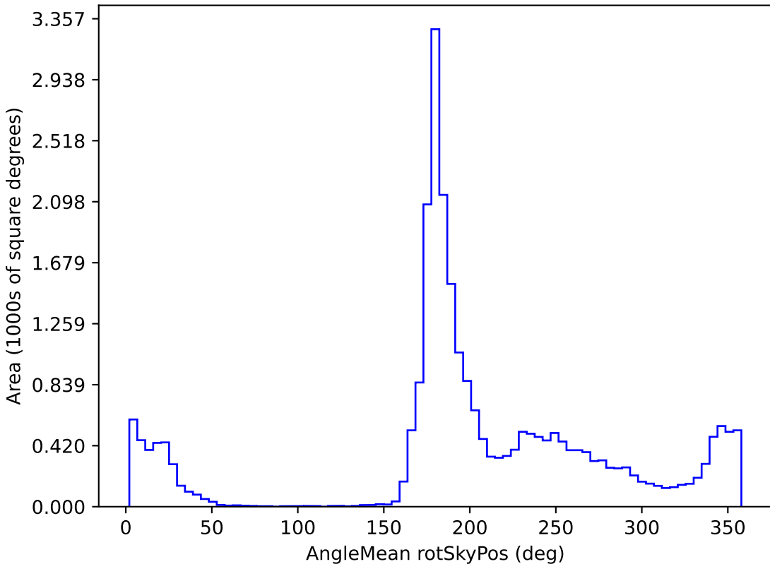
too_5_4v3.4_10yrs All sky all bands: AngleMean rotSkyPos
