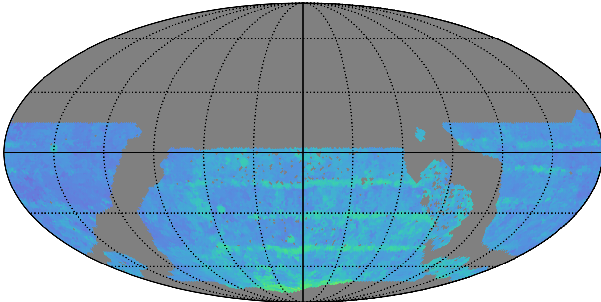
too_5_4v3.4_10yrs WFD z band: 80thPercentile Season Length
