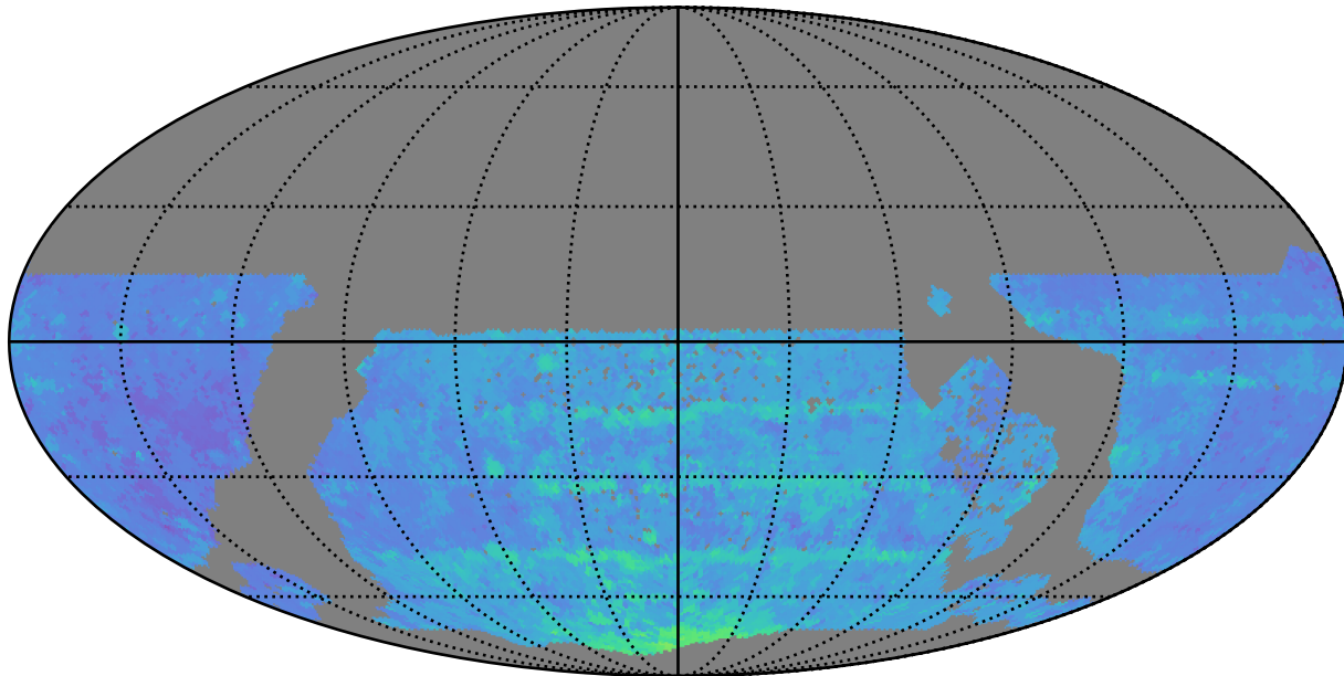
too_5_4v3.4_10yrs WFD y band: 80thPercentile Season Length
