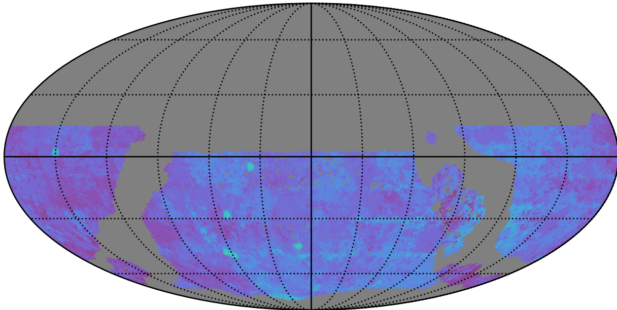
too_5_4v3.4_10yrs WFD u band: 80thPercentile Season Length
