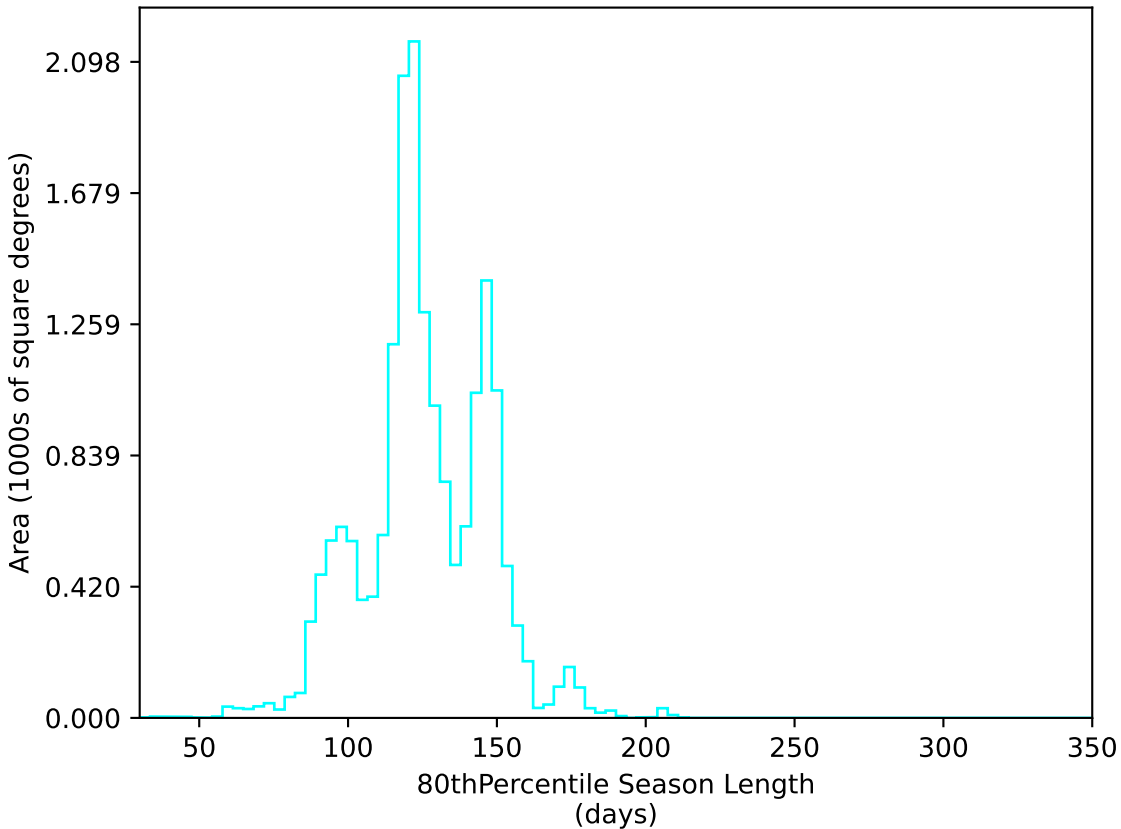
too_5_4v3.4_10yrs WFD u band: 80thPercentile Season Length
