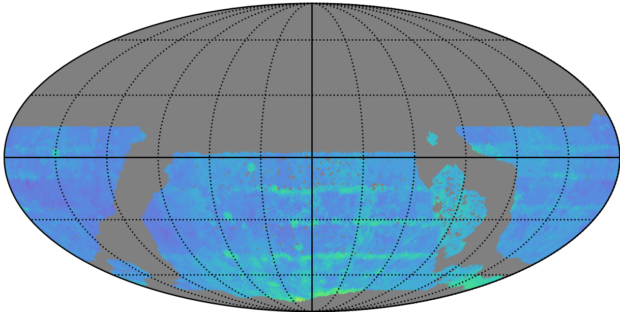
too_5_4v3.4_10yrs WFD r band: 80thPercentile Season Length
