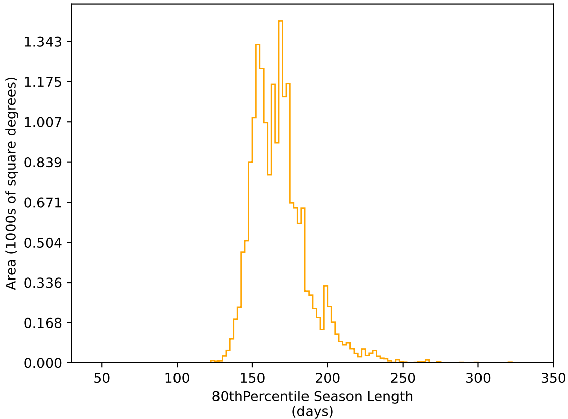
too_5_4v3.4_10yrs WFD r band: 80thPercentile Season Length
