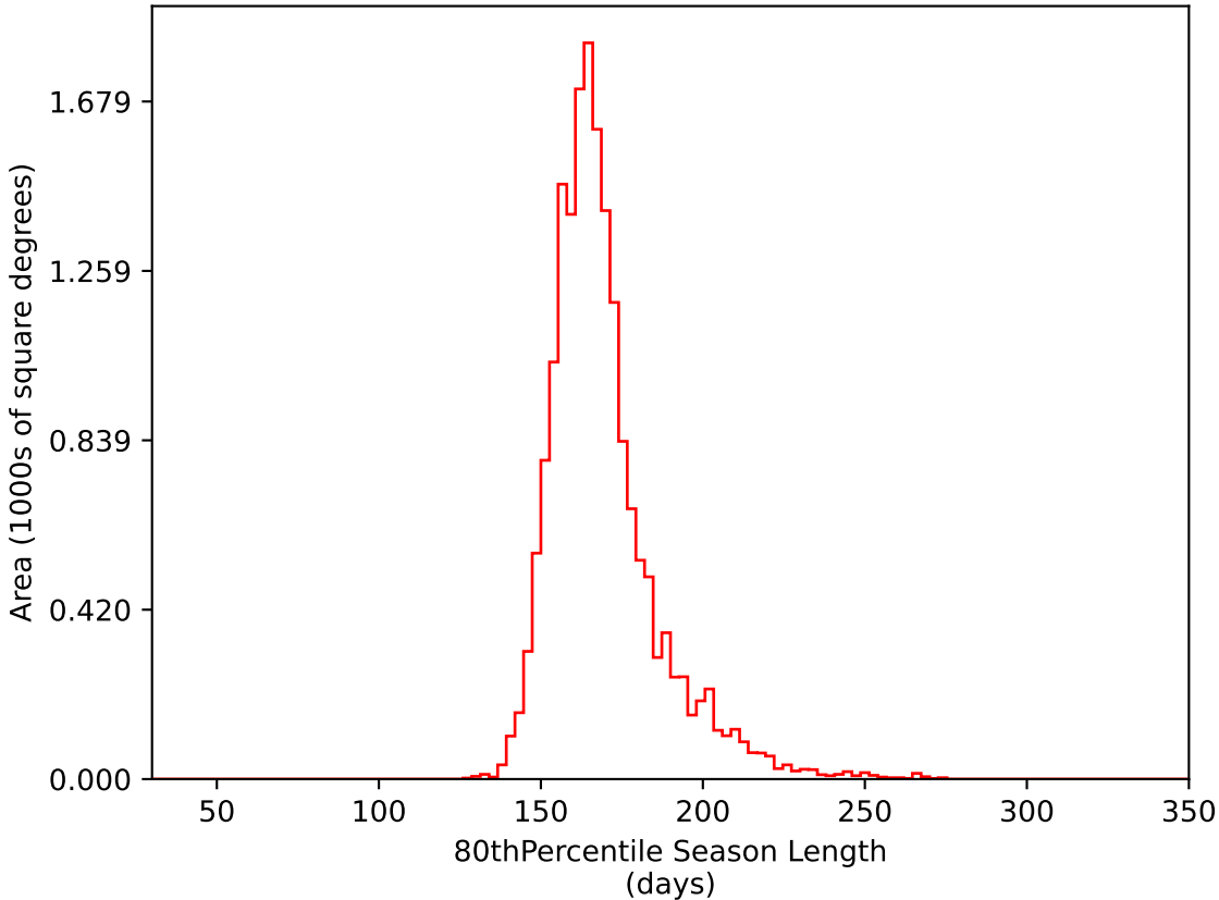
too_5_4v3.4_10yrs WFD i band: 80thPercentile Season Length
