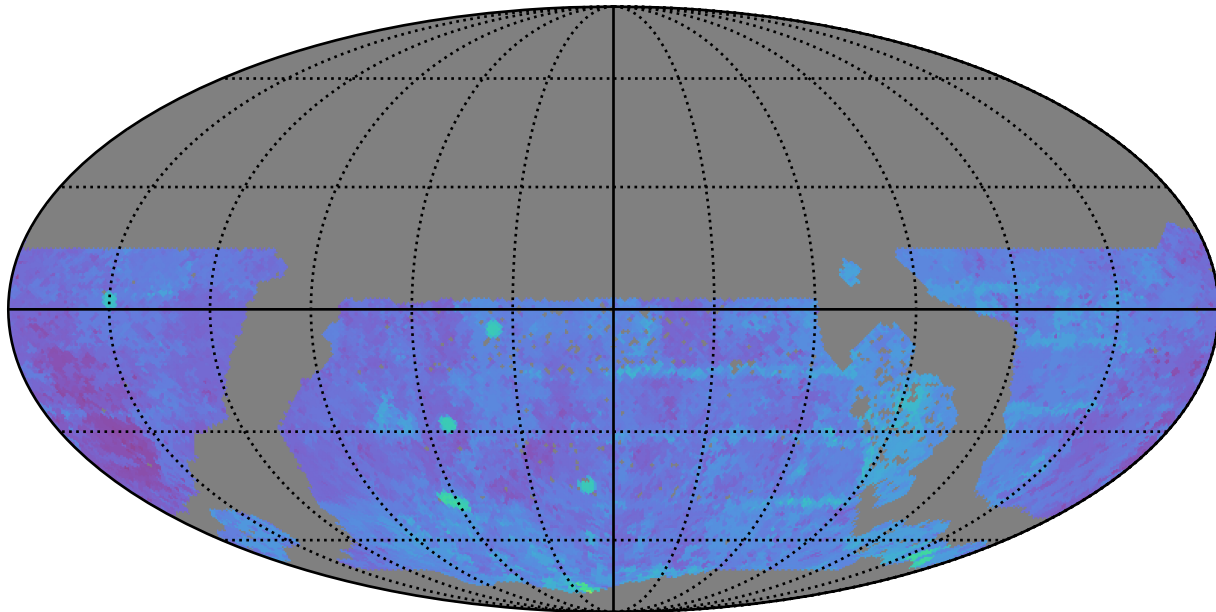
too_5_4v3.4_10yrs WFD g band: 80thPercentile Season Length
