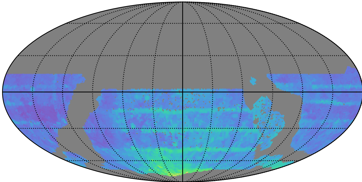
too_5_4v3.4_10yrs WFD all bands: 80thPercentile Season Length
