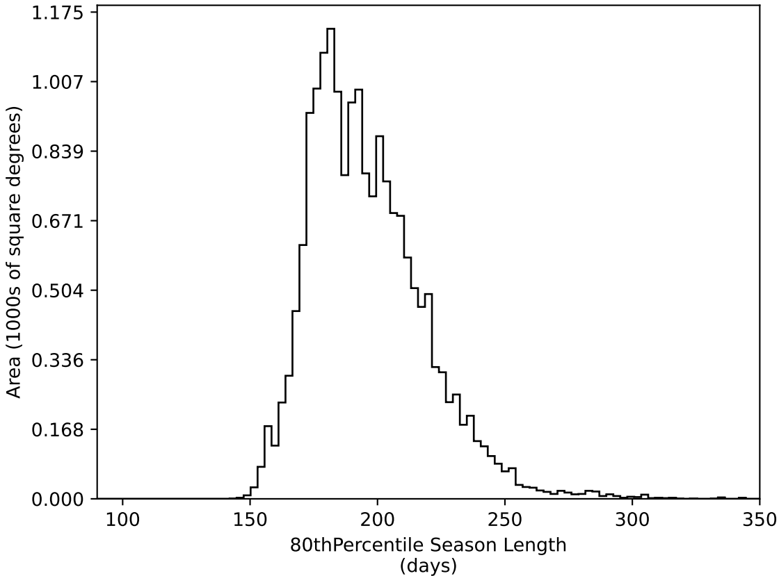
too_5_4v3.4_10yrs WFD all bands: 80thPercentile Season Length
