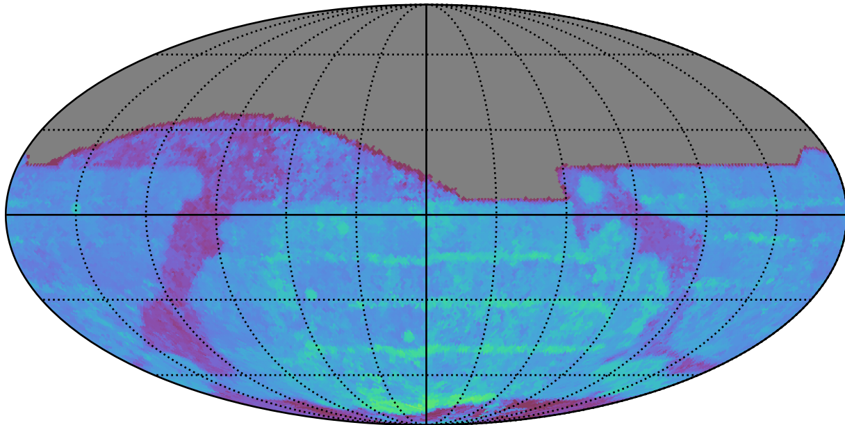
too_5_4v3.4_10yrs All sky z band: 80thPercentile Season Length
