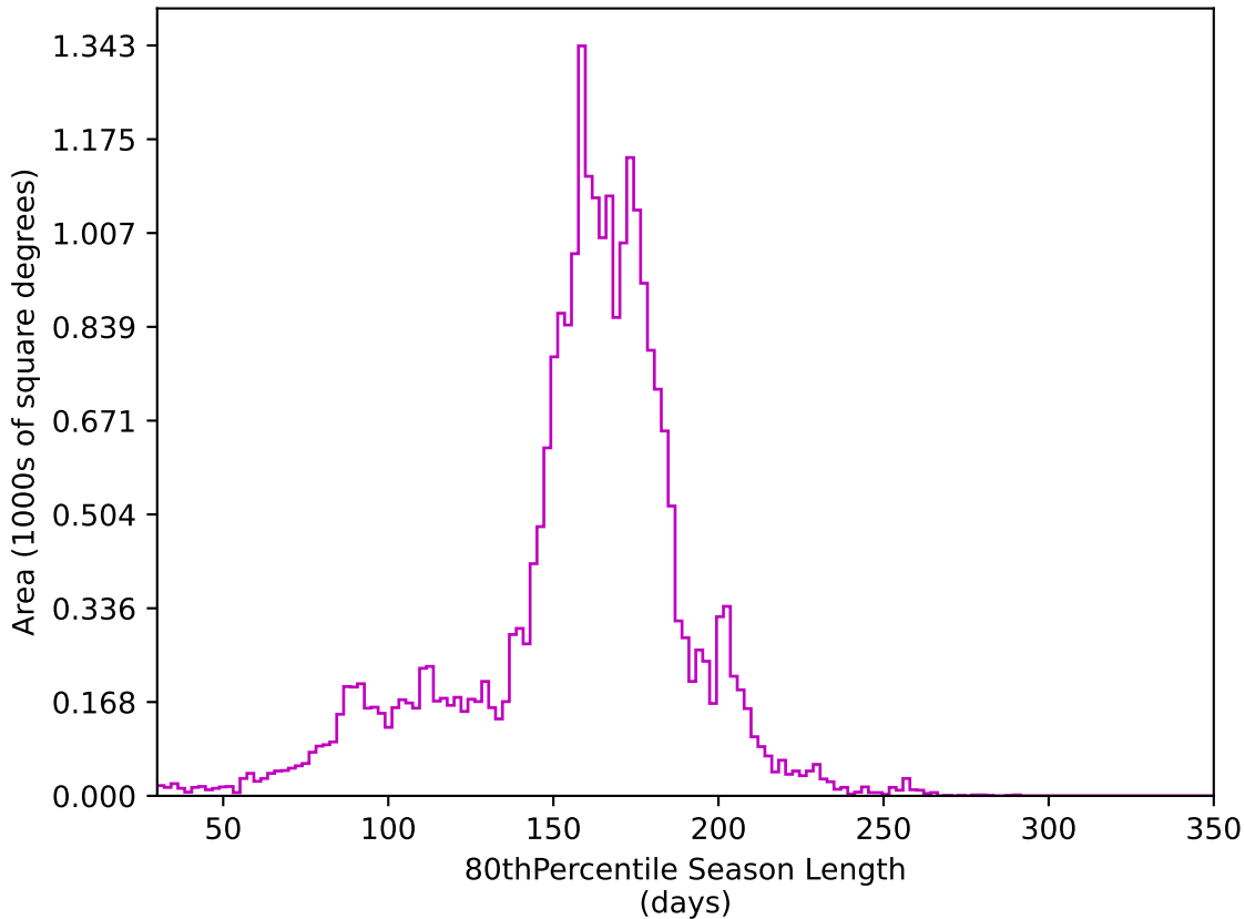
too_5_4v3.4_10yrs All sky z band: 80thPercentile Season Length
