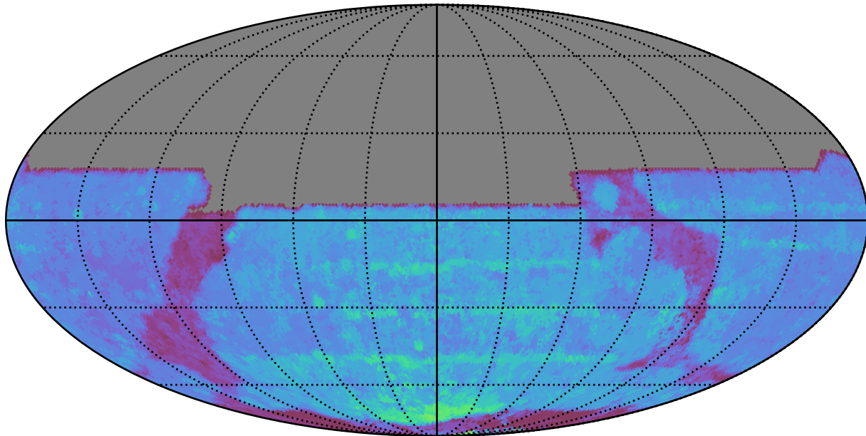
too_5_4v3.4_10yrs All sky y band: 80thPercentile Season Length
