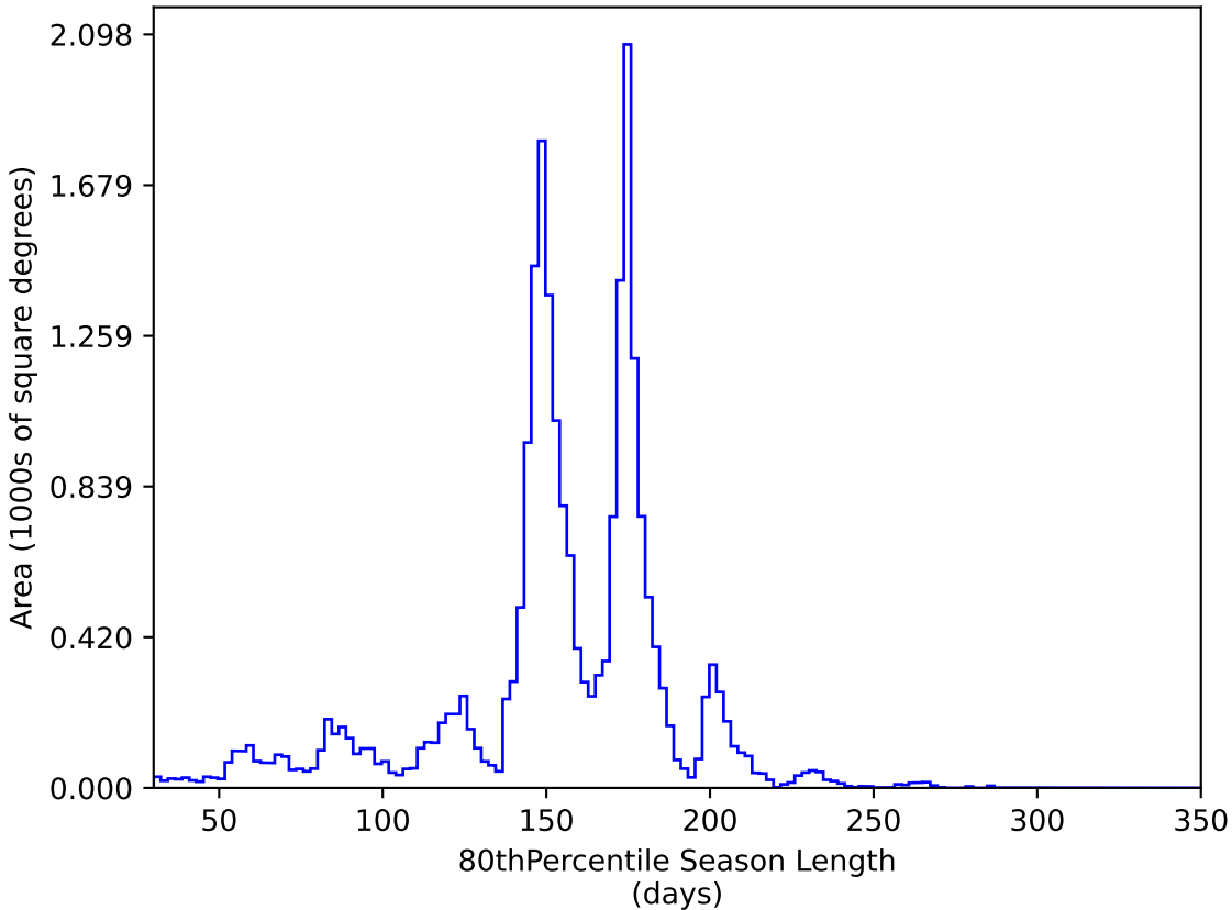
too_5_4v3.4_10yrs All sky y band: 80thPercentile Season Length
