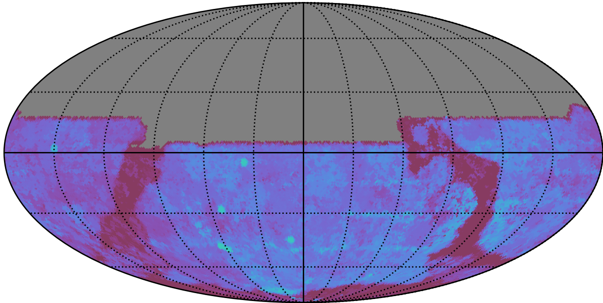
too_5_4v3.4_10yrs All sky u band: 80thPercentile Season Length
