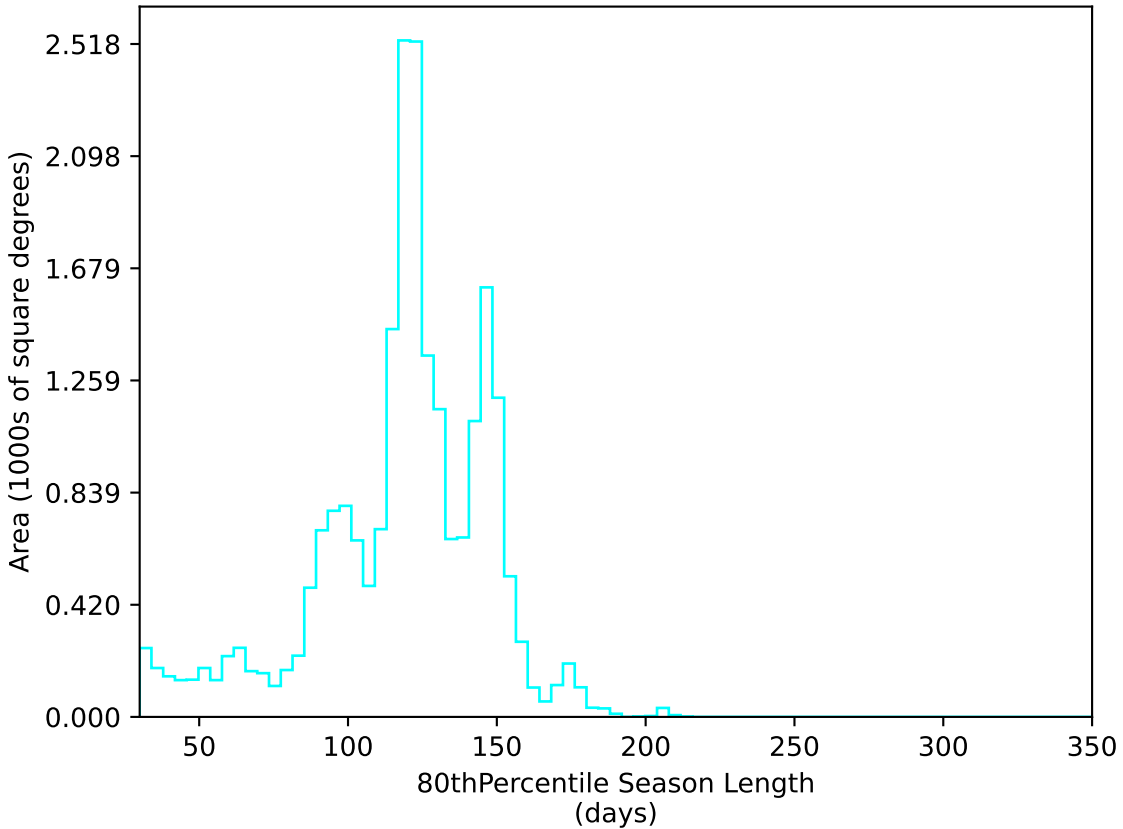
too_5_4v3.4_10yrs All sky u band: 80thPercentile Season Length
