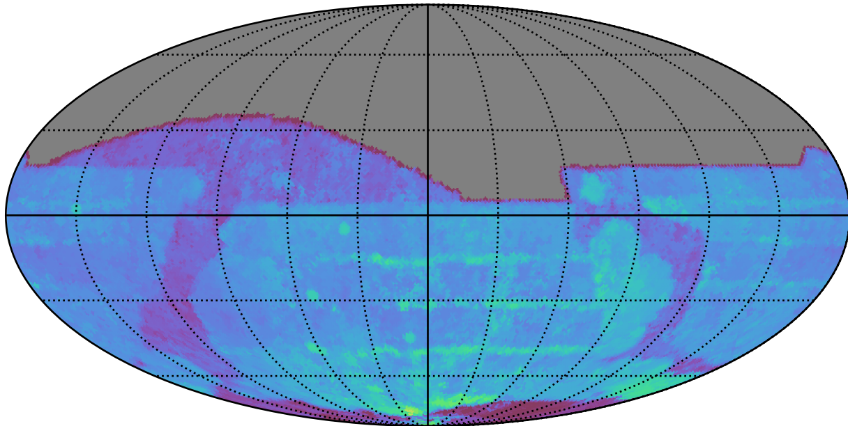
too_5_4v3.4_10yrs All sky r band: 80thPercentile Season Length
