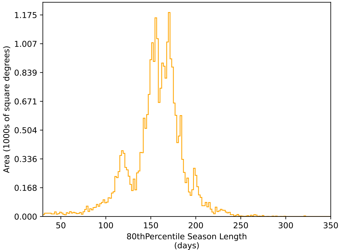
too_5_4v3.4_10yrs All sky r band: 80thPercentile Season Length
