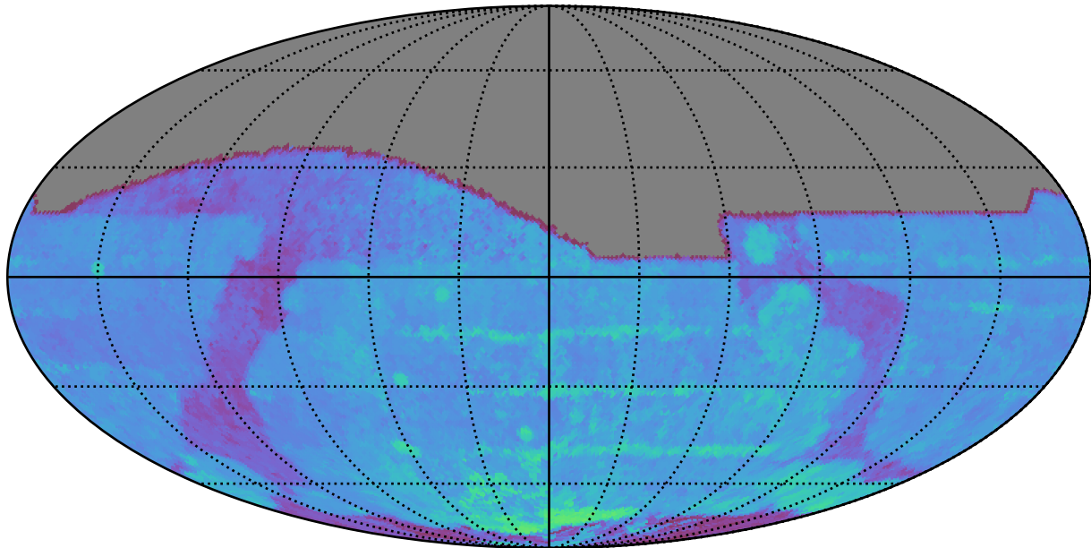
too_5_4v3.4_10yrs All sky i band: 80thPercentile Season Length
