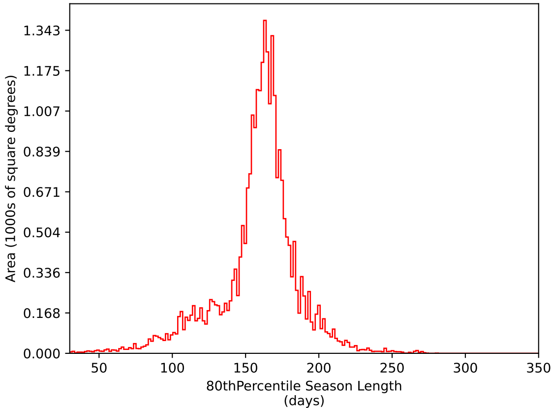
too_5_4v3.4_10yrs All sky i band: 80thPercentile Season Length
