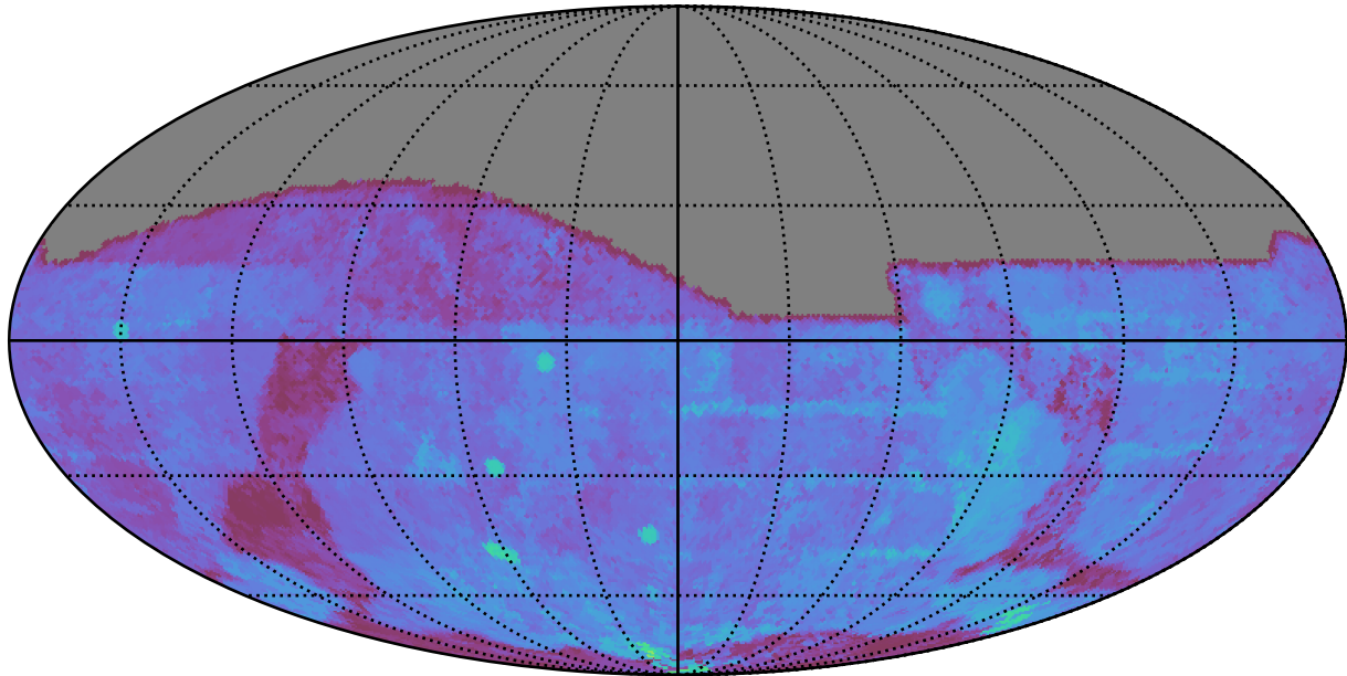
too_5_4v3.4_10yrs All sky g band: 80thPercentile Season Length
