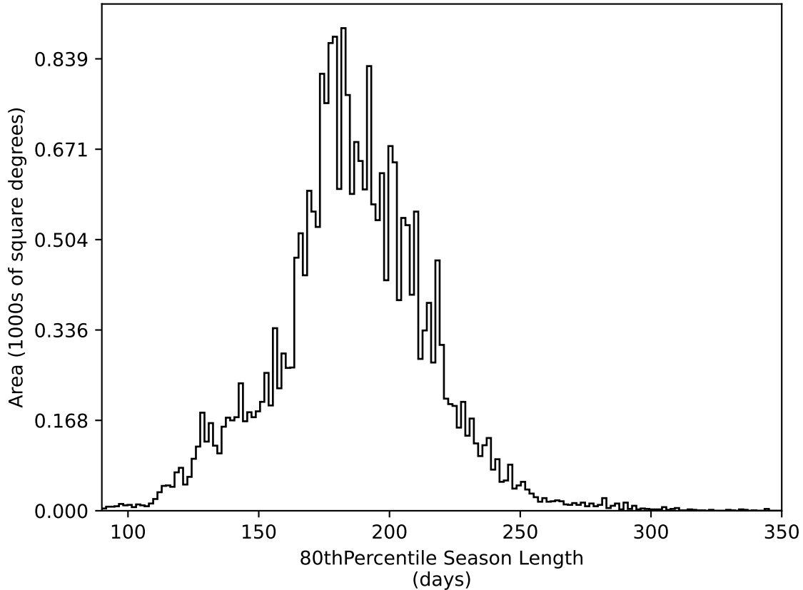
too_5_4v3.4_10yrs All sky all bands: 80thPercentile Season Length
