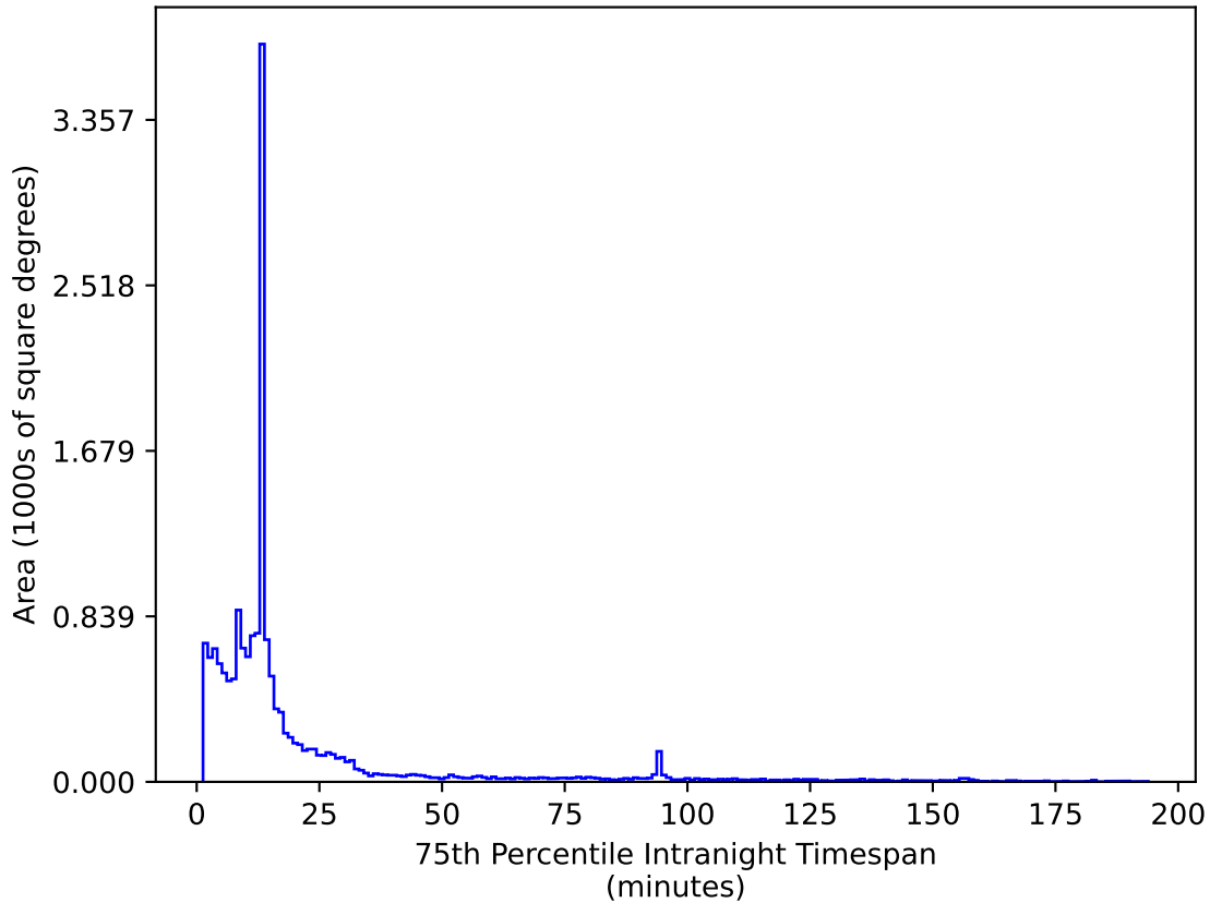
too_5_4v3.4_10yrs WFD z band: 75th Percentile Intranight Timespan
